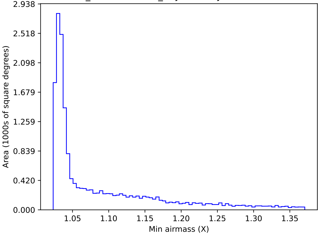
weather_cloudso12v3.4_10yrs WFD y band: Min airmass
