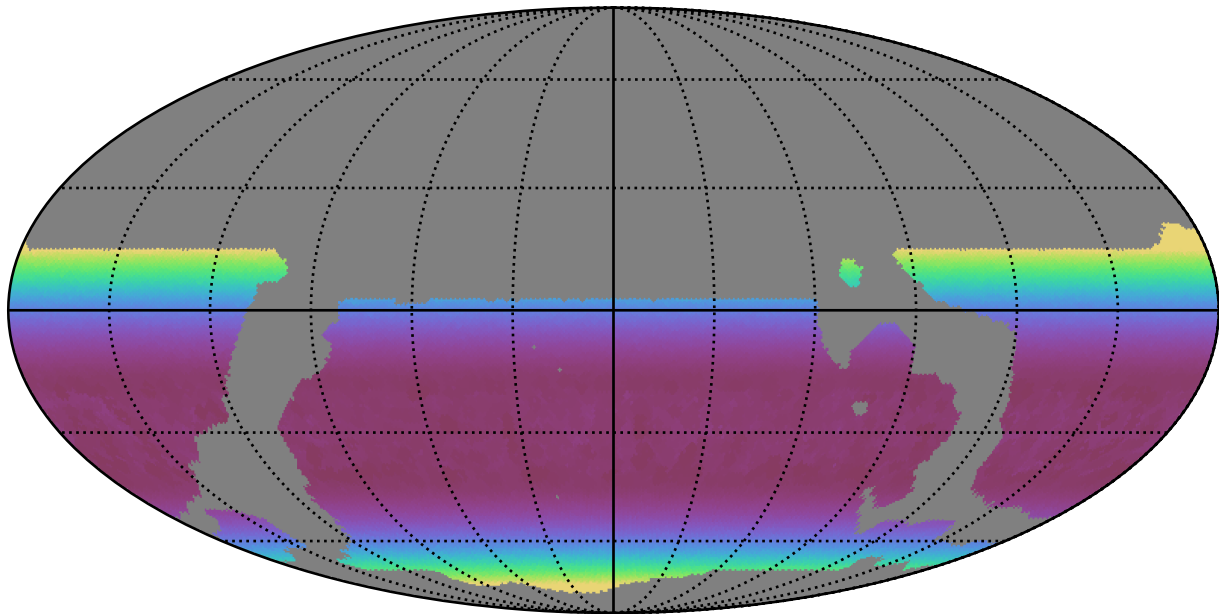
weather_cloudso12v3.4_10yrs WFD i band: Min airmass
