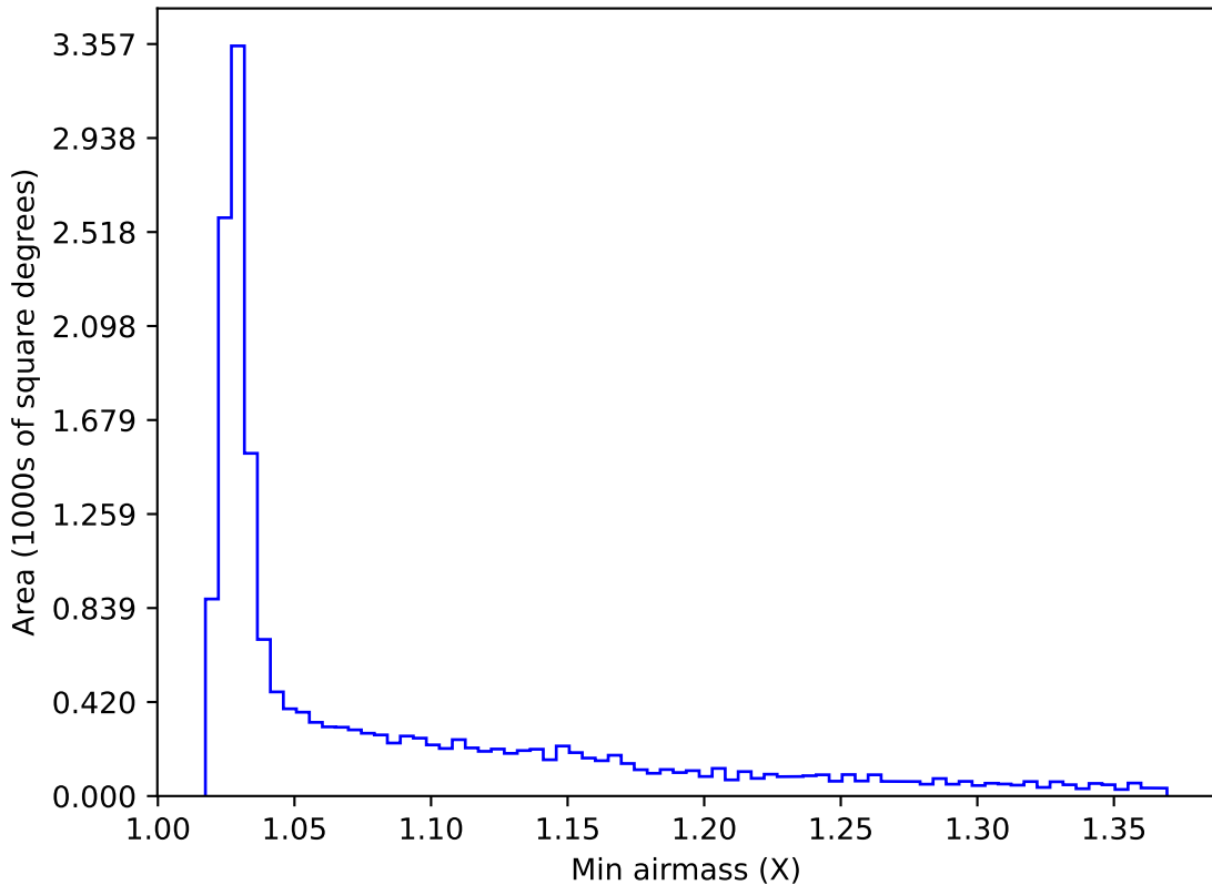
weather_cloudso12v3.4_10yrs WFD i band: Min airmass
