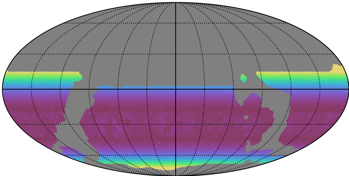
weather_cloudso12v3.4_10yrs WFD g band: Min airmass
