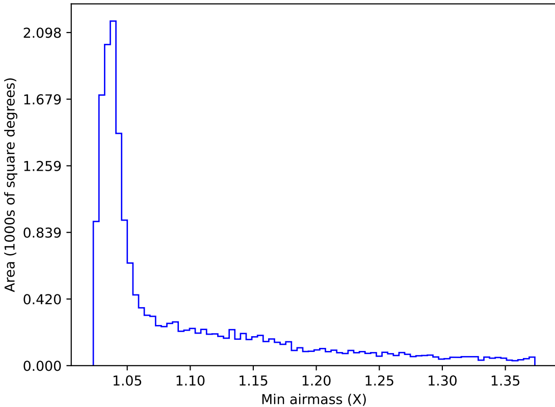
weather_cloudso12v3.4_10yrs WFD g band: Min airmass
