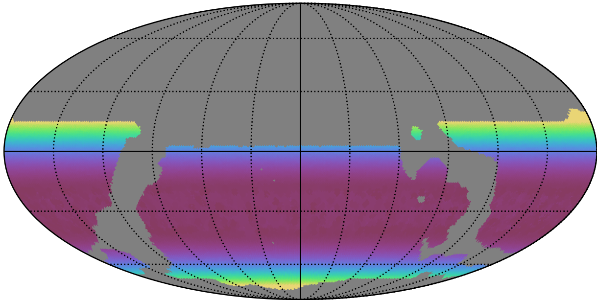
weather_cloudso12v3.4_10yrs WFD all bands: Min airmass
