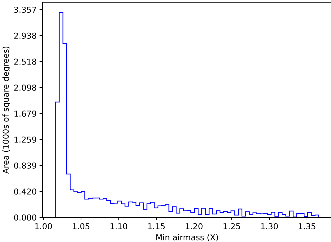
weather_cloudso12v3.4_10yrs WFD all bands: Min airmass
