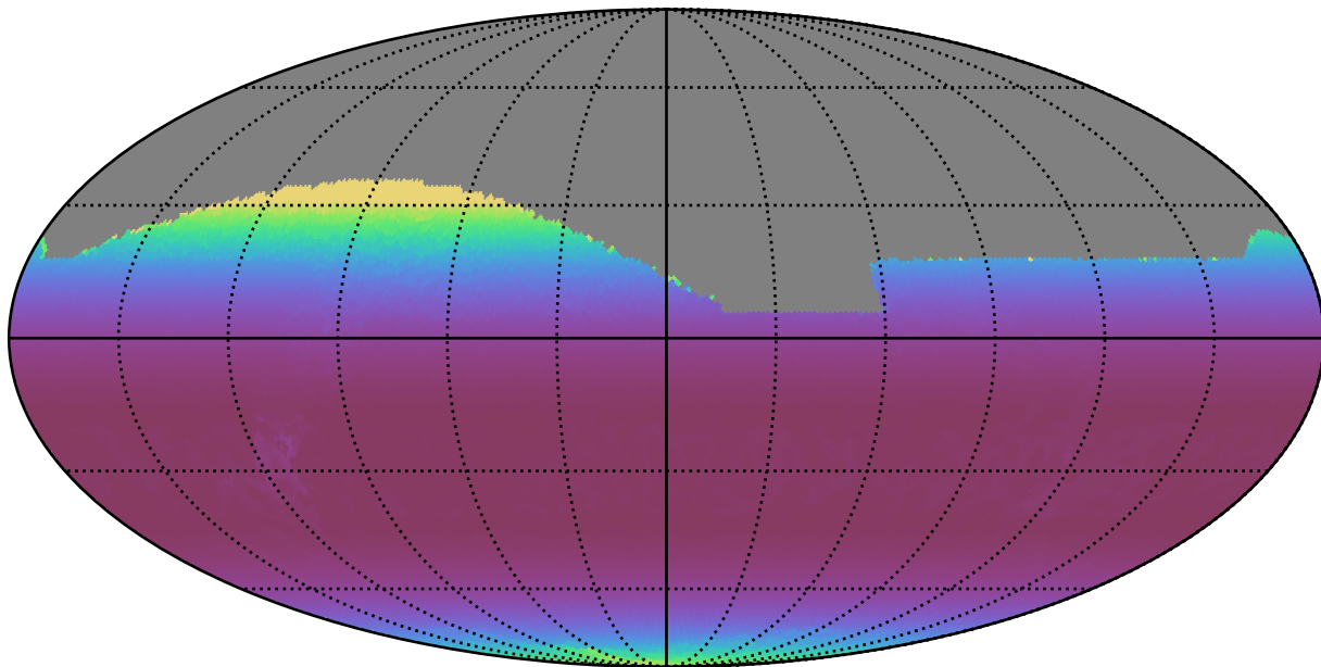
weather_cloudso12v3.4_10yrs All sky z band: Min airmass
