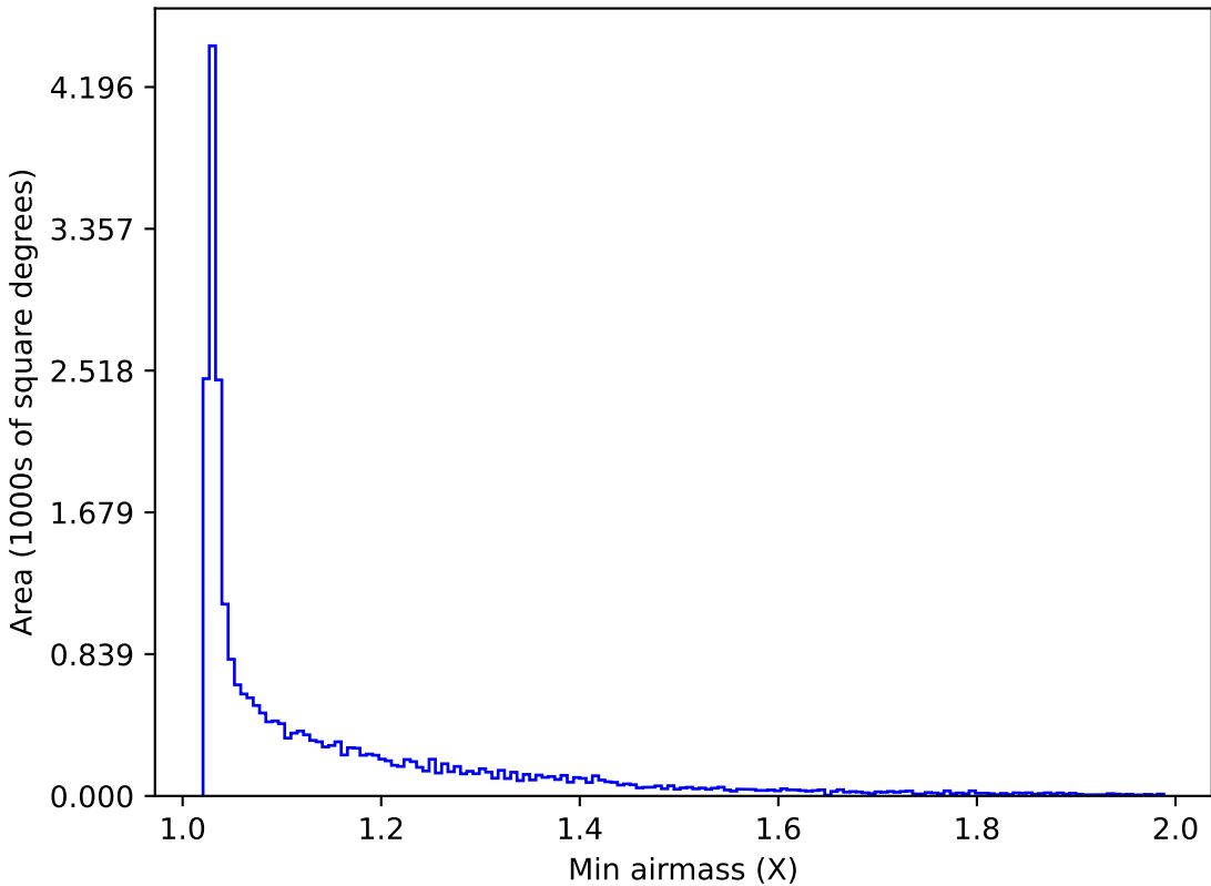
weather_cloudso12v3.4_10yrs All sky z band: Min airmass
