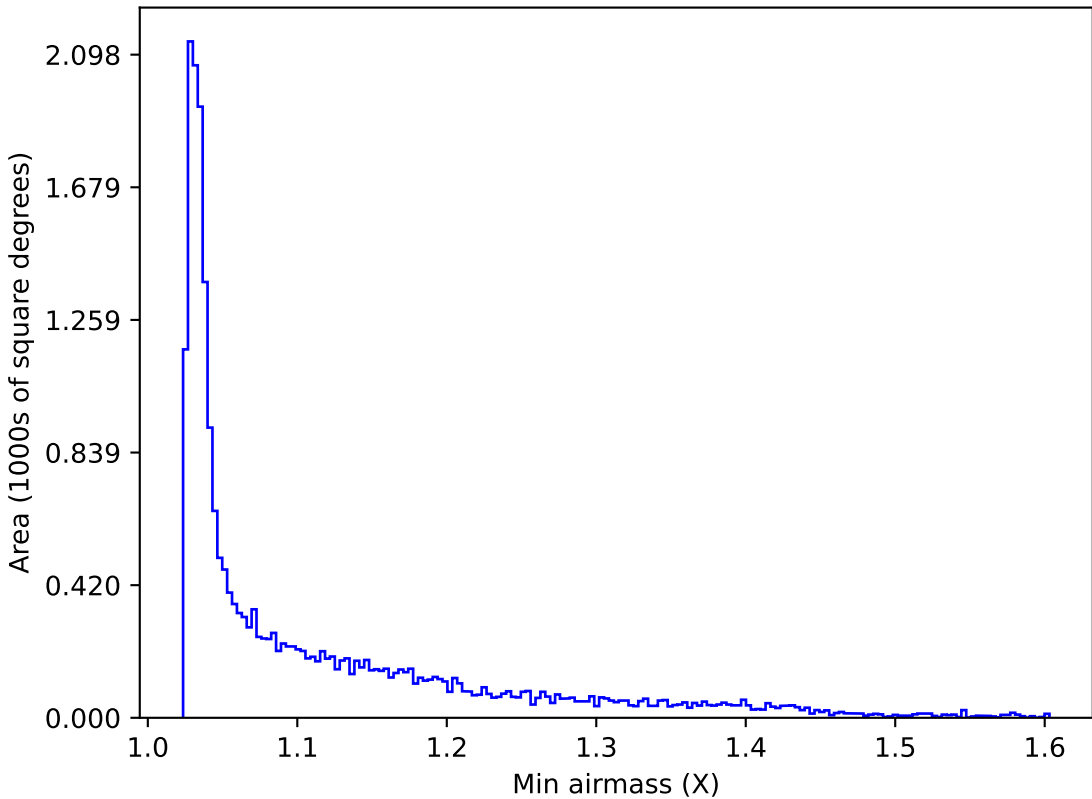
weather_cloudso12v3.4_10yrs All sky y band: Min airmass
