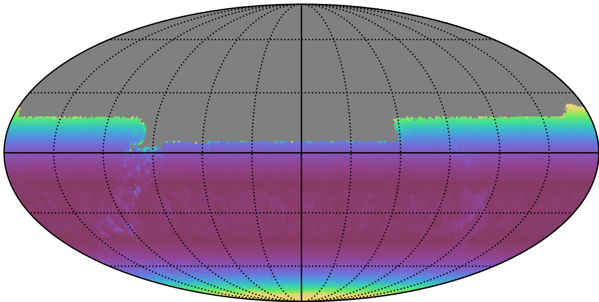
weather_cloudso12v3.4_10yrs All sky u band: Min airmass
