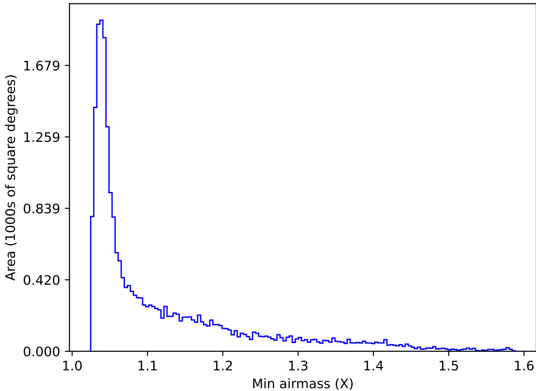
weather_cloudso12v3.4_10yrs All sky u band: Min airmass
