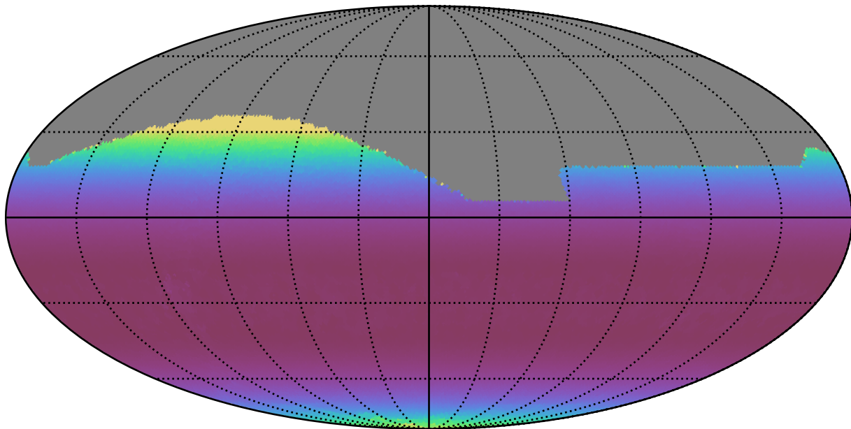
weather_cloudso12v3.4_10yrs All sky r band: Min airmass
