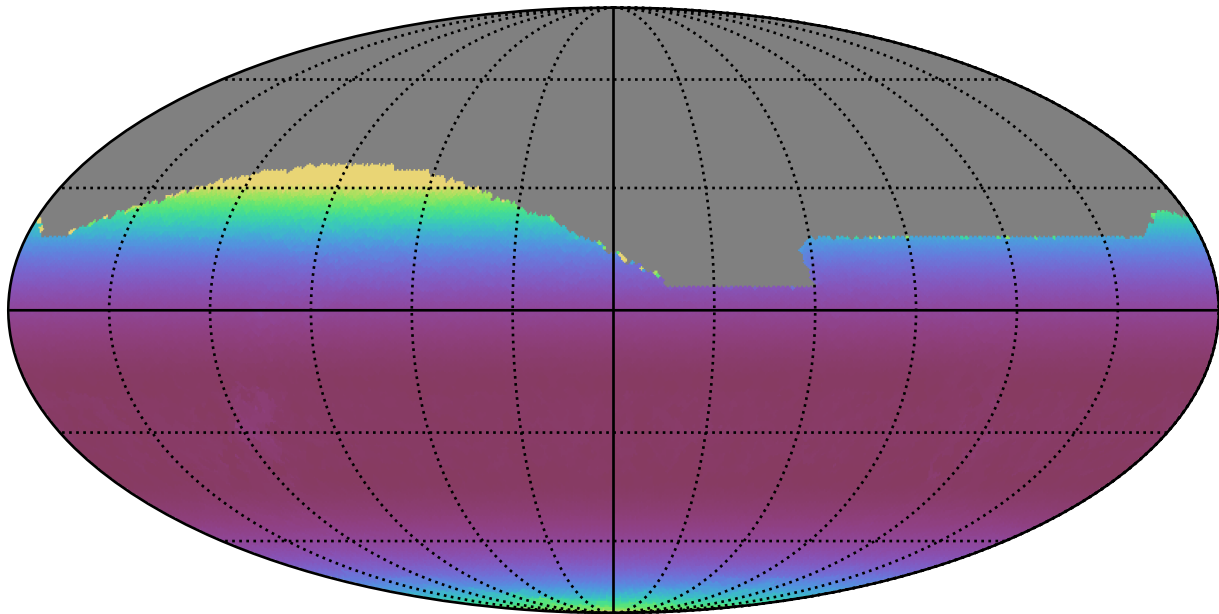
weather_cloudso12v3.4_10yrs All sky i band: Min airmass
