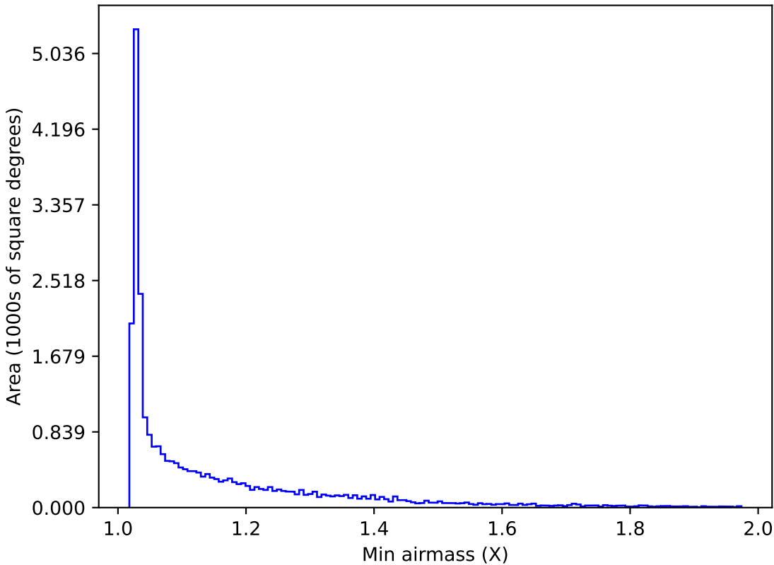
weather_cloudso12v3.4_10yrs All sky i band: Min airmass
