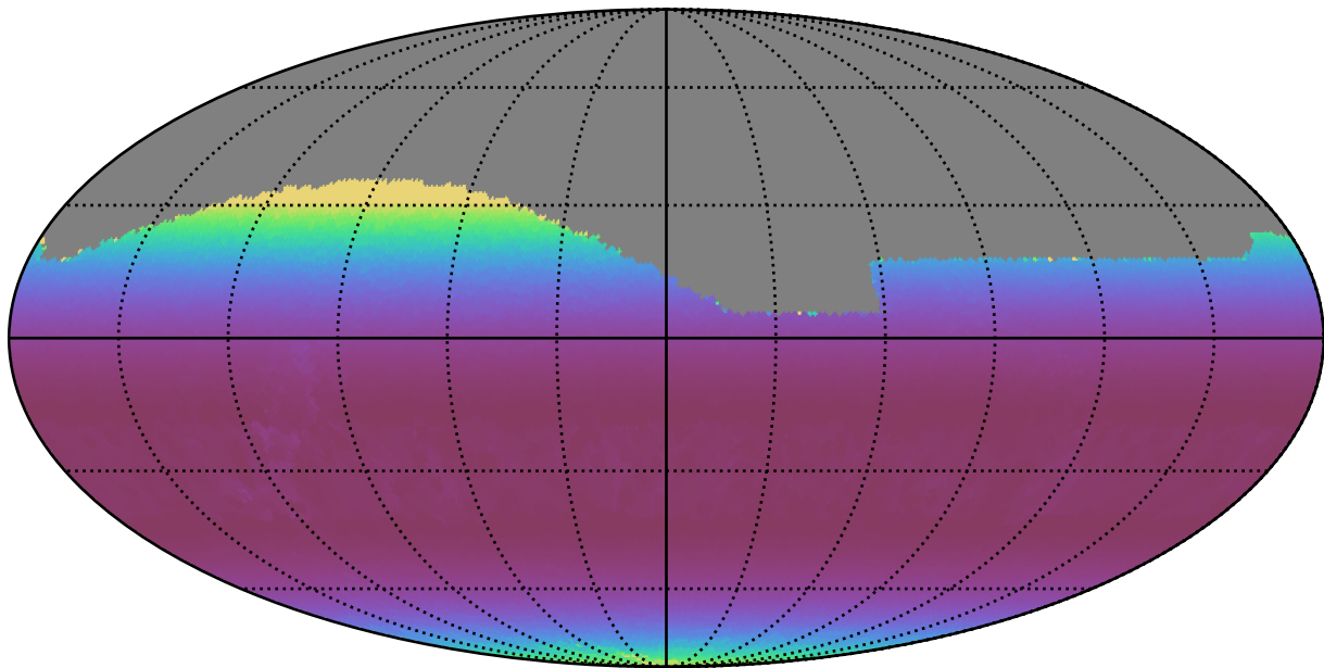
weather_cloudso12v3.4_10yrs All sky g band: Min airmass
