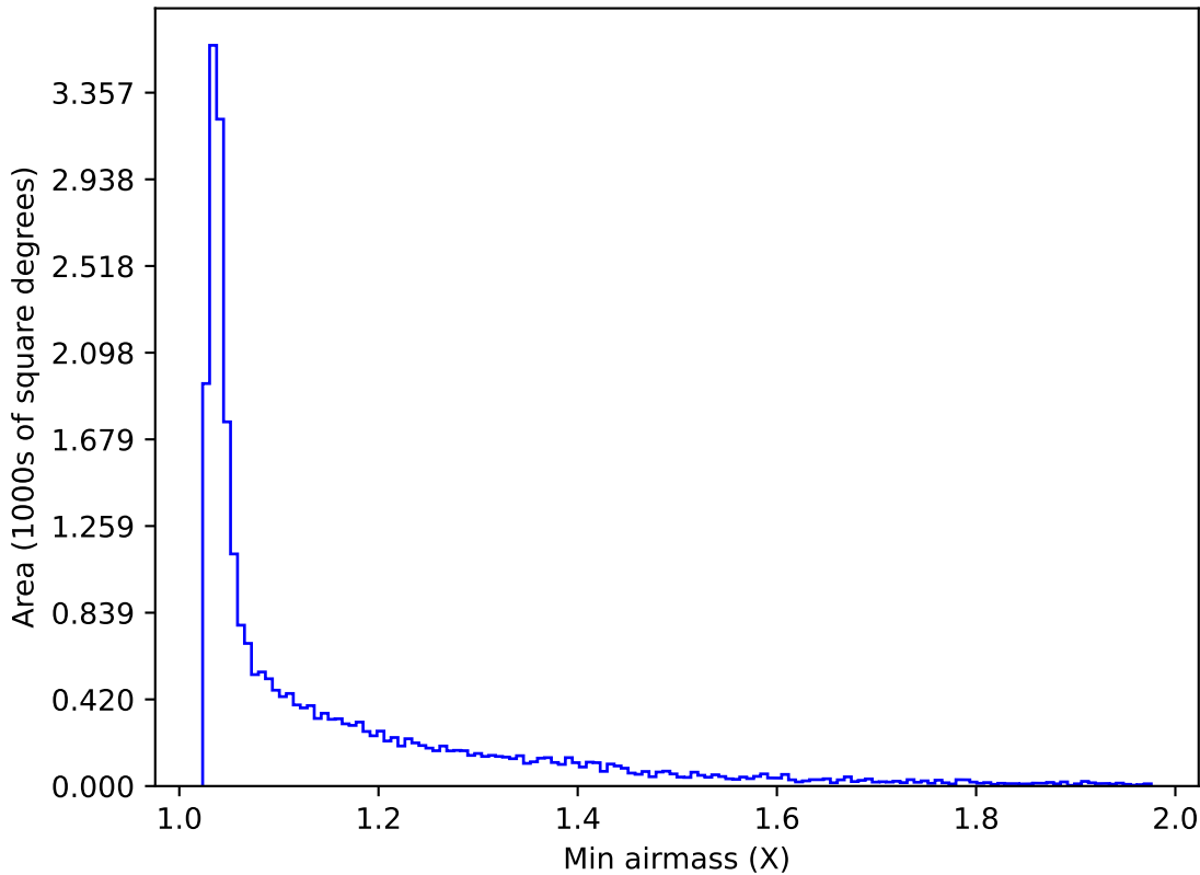
weather_cloudso12v3.4_10yrs All sky g band: Min airmass
