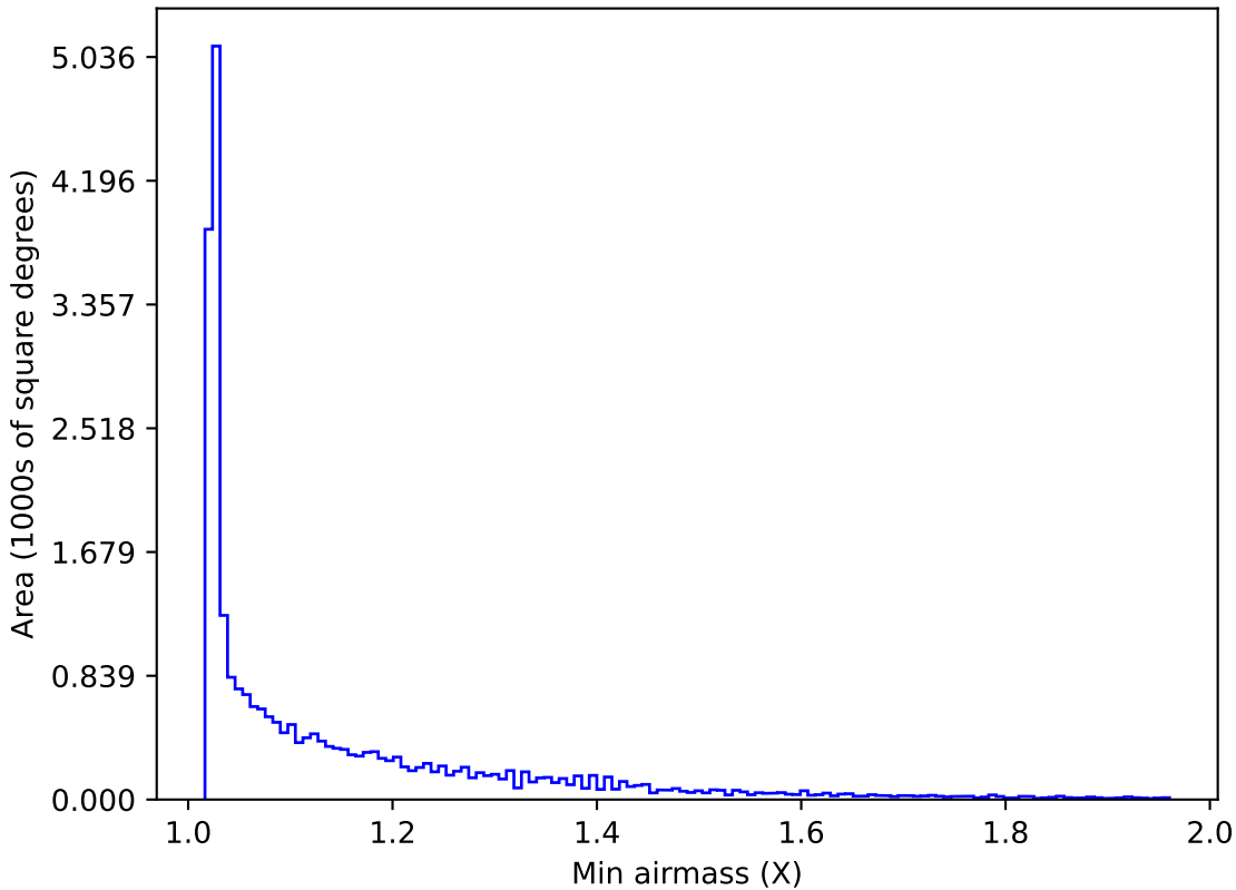
weather_cloudso12v3.4_10yrs All sky all bands: Min airmass
