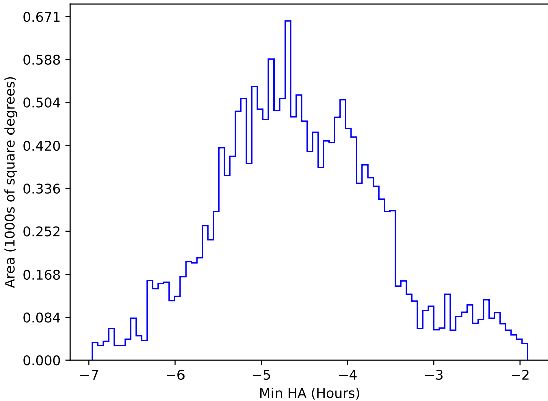
weather_cloudso12v3.4_10yrs WFD z band: Min HA
