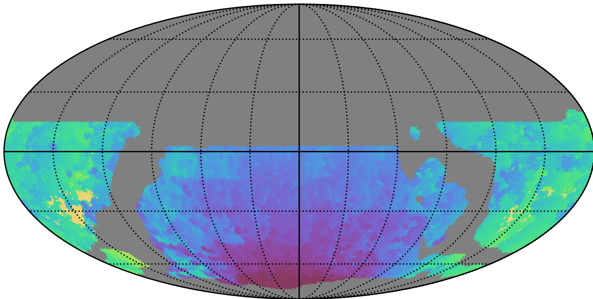
weather_cloudso12v3.4_10yrs WFD y band: Min HA
