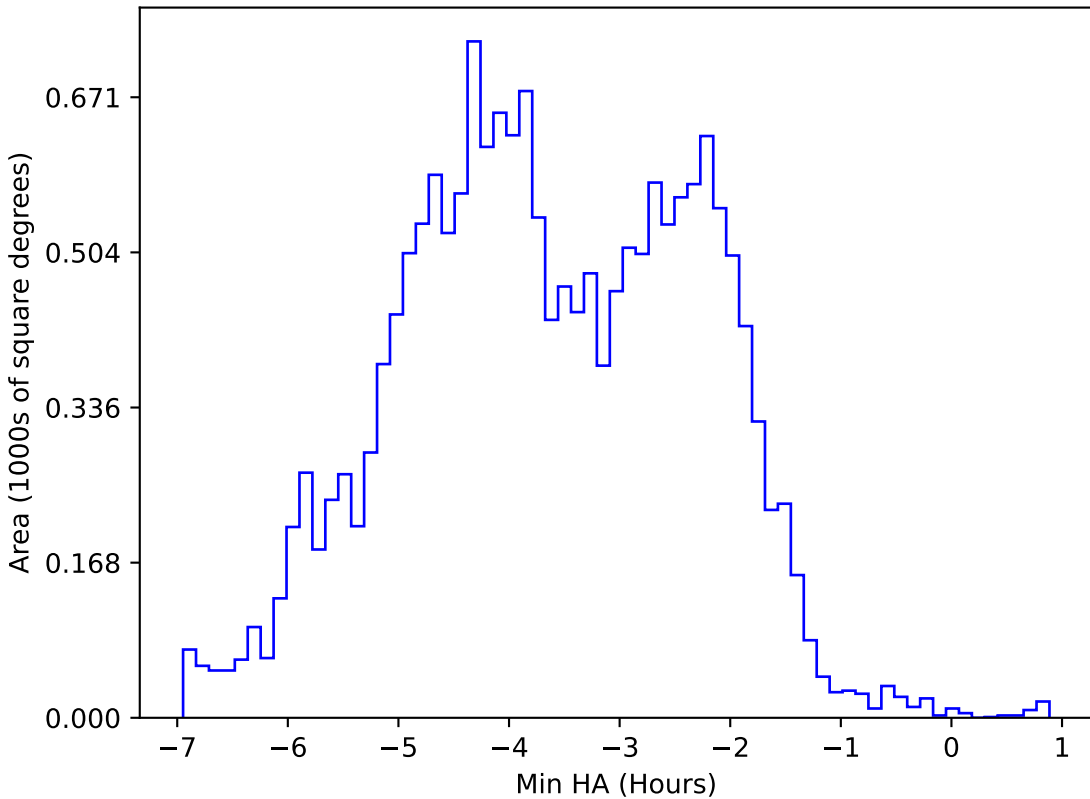
weather_cloudso12v3.4_10yrs WFD y band: Min HA
