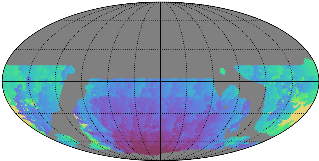
weather_cloudso12v3.4_10yrs WFD u band: Min HA
