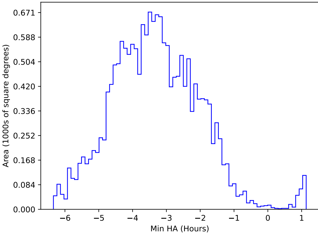
weather_cloudso12v3.4_10yrs WFD u band: Min HA
