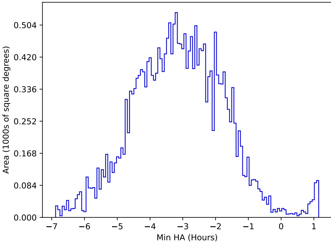
weather_cloudso12v3.4_10yrs All sky u band: Min HA
