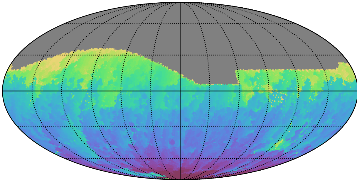
weather_cloudso12v3.4_10yrs All sky g band: Min HA
