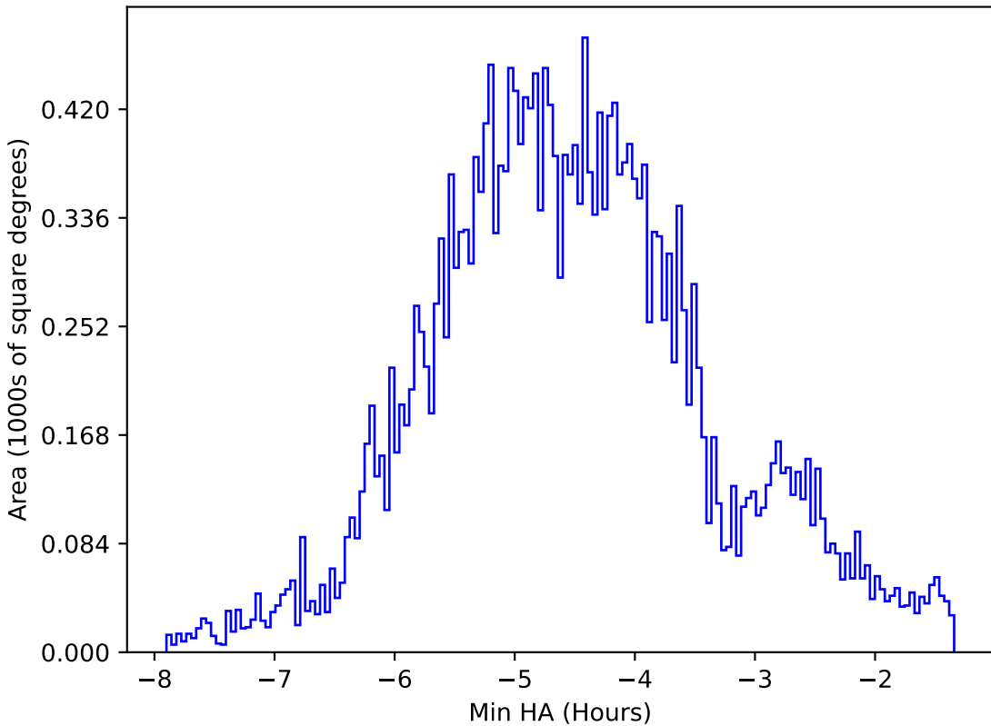
weather_cloudso12v3.4_10yrs All sky all bands: Min HA
