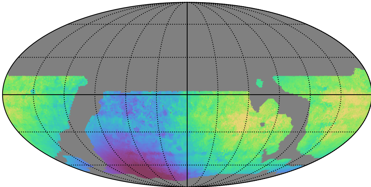
weather_cloudso12v3.4_10yrs WFD z band: Median solarElong
