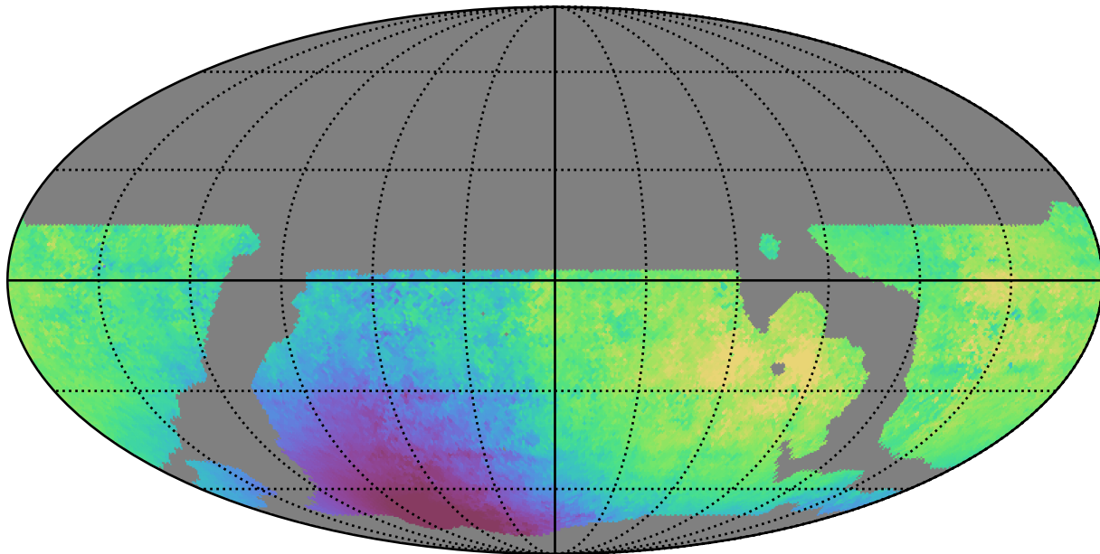
weather_cloudso12v3.4_10yrs WFD y band: Median solarElong
