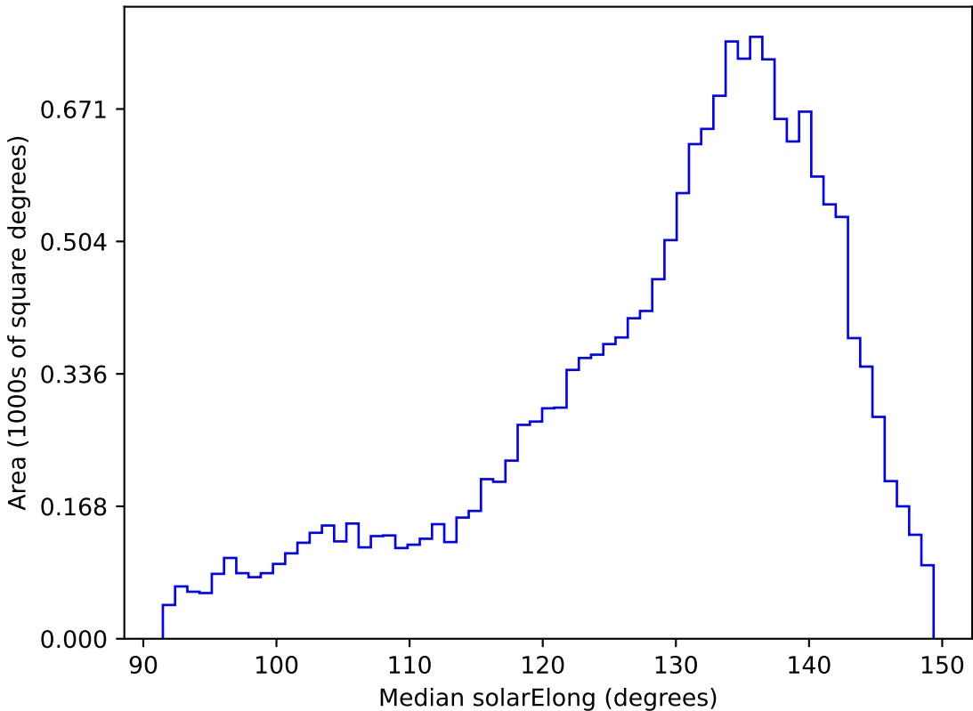
weather_cloudso12v3.4_10yrs WFD y band: Median solarElong
