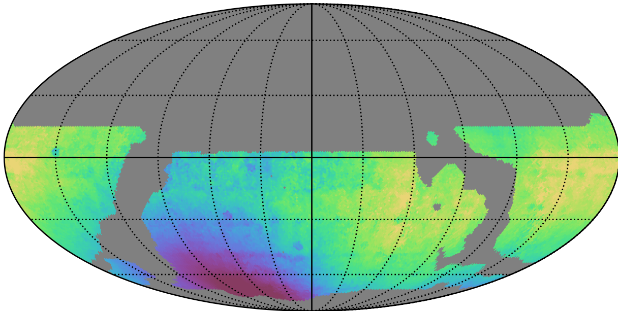
weather_cloudso12v3.4_10yrs WFD r band: Median solarElong
