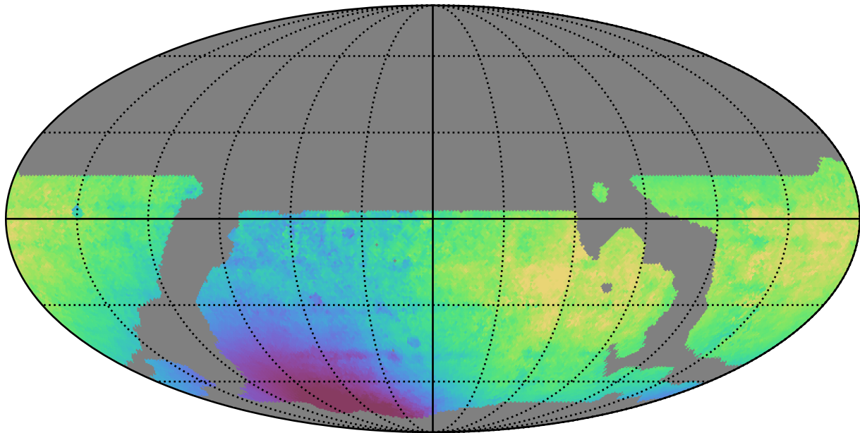
weather_cloudso12v3.4_10yrs WFD i band: Median solarElong
