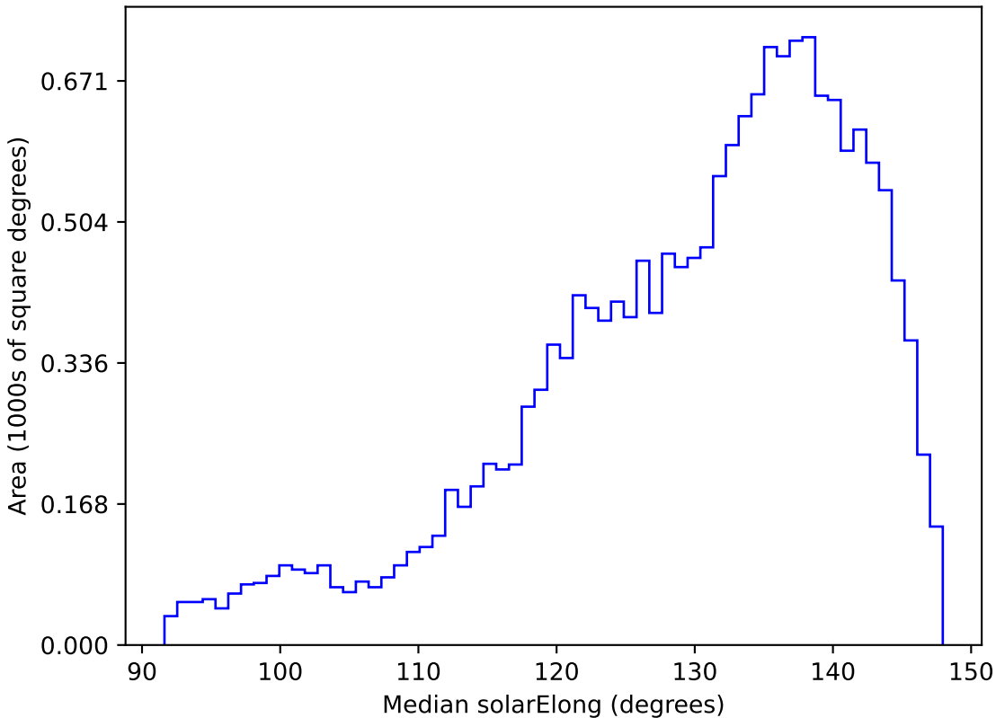
weather_cloudso12v3.4_10yrs WFD i band: Median solarElong
