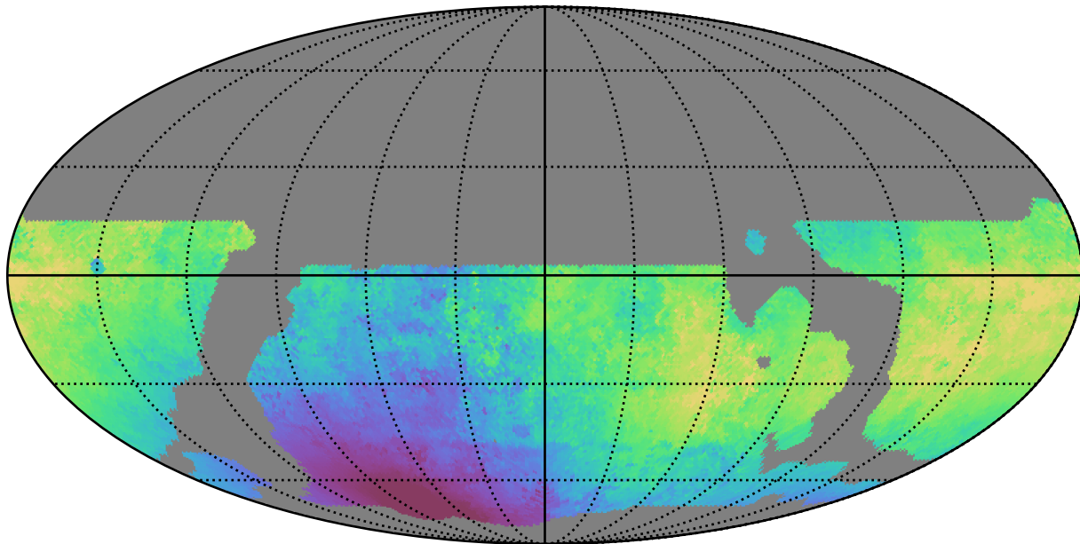
weather_cloudso12v3.4_10yrs WFD g band: Median solarElong
