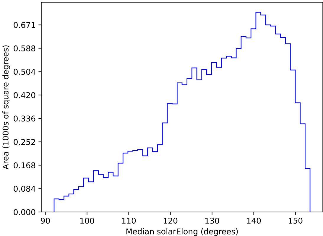
weather_cloudso12v3.4_10yrs WFD g band: Median solarElong
