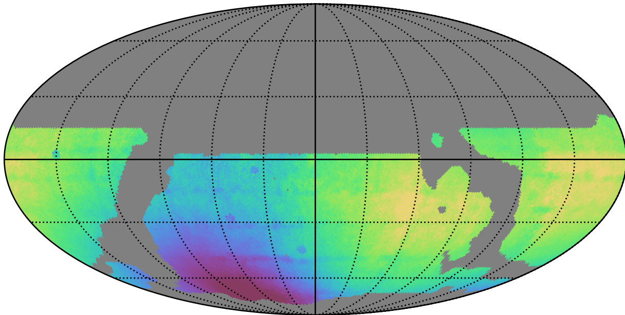
weather_cloudso12v3.4_10yrs WFD all bands: Median solarElong
