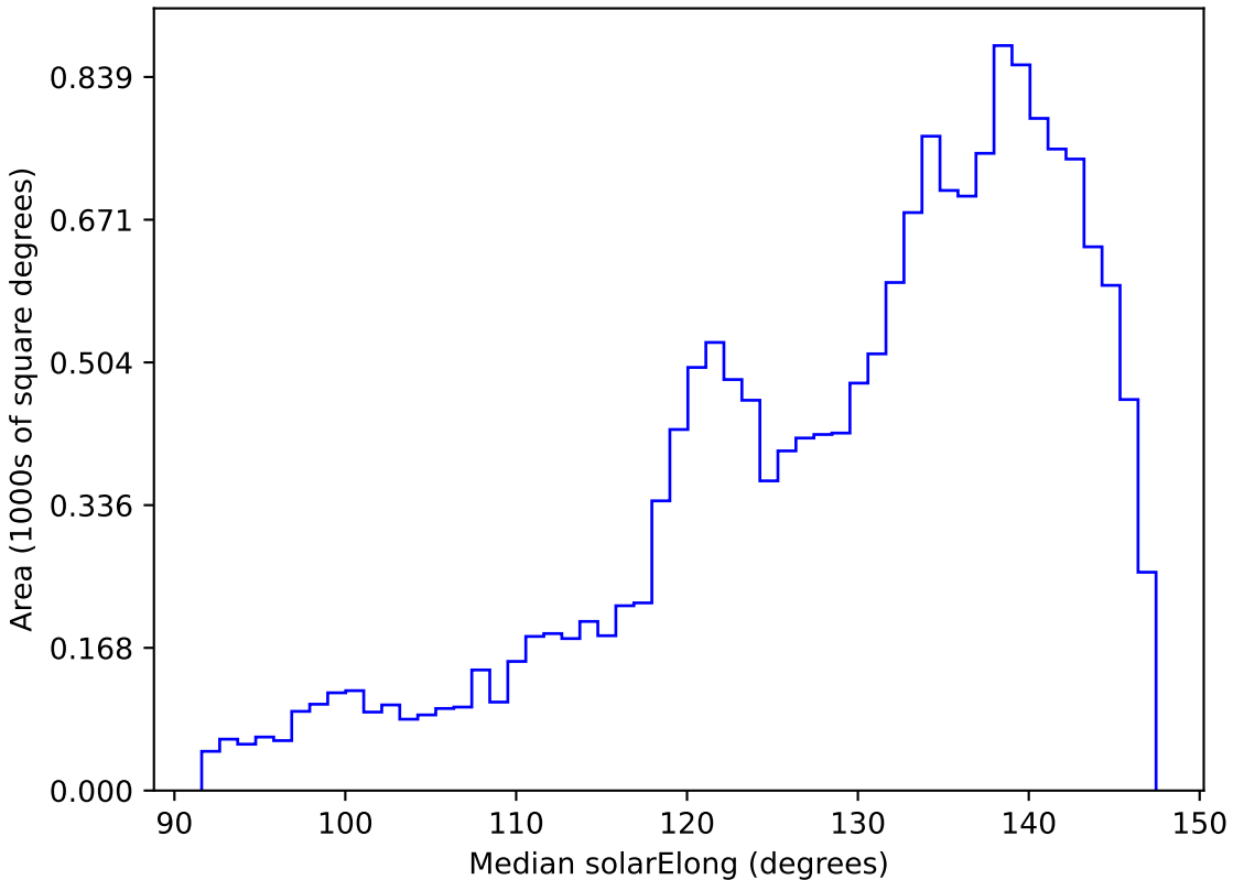
weather_cloudso12v3.4_10yrs WFD all bands: Median solarElong
