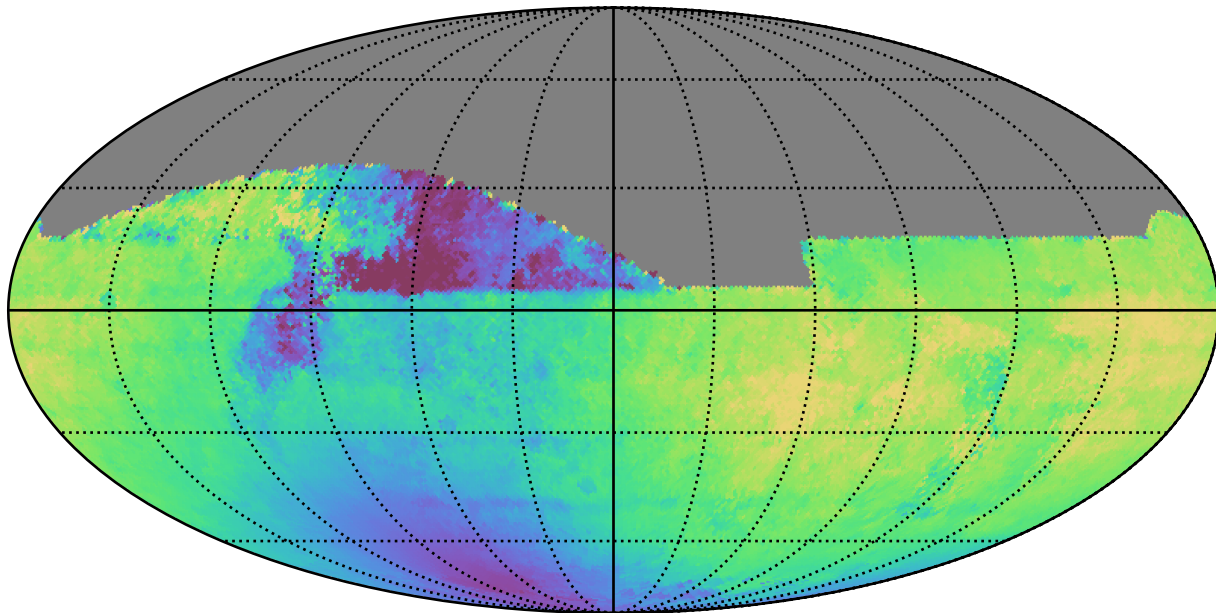
weather_cloudso12v3.4_10yrs All sky z band: Median solarElong
