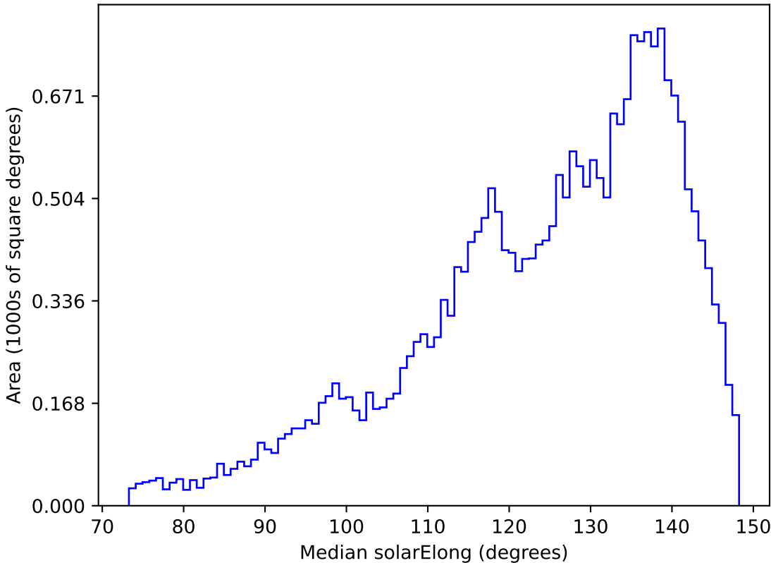
weather_cloudso12v3.4_10yrs All sky z band: Median solarElong
