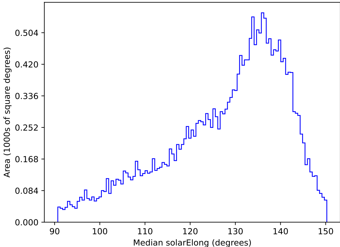
weather_cloudso12v3.4_10yrs All sky y band: Median solarElong
