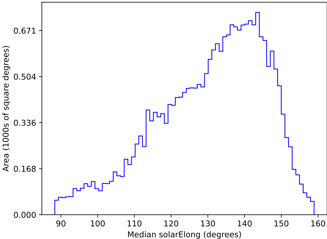
weather_cloudso12v3.4_10yrs All sky u band: Median solarElong
