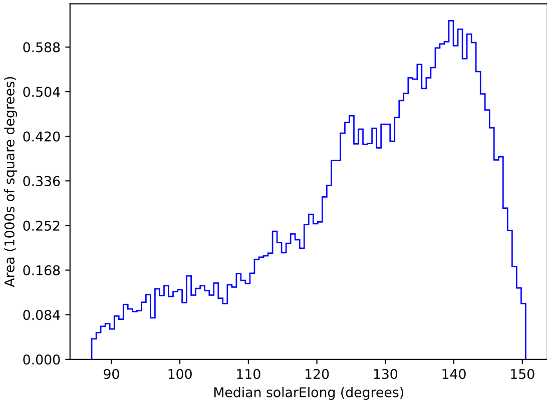
weather_cloudso12v3.4_10yrs All sky r band: Median solarElong
