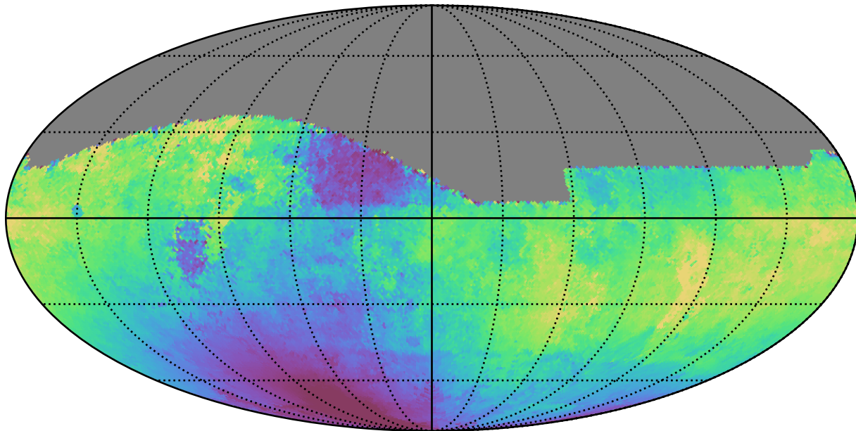
weather_cloudso12v3.4_10yrs All sky g band: Median solarElong
