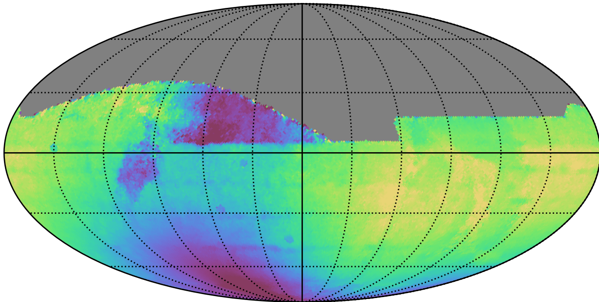
weather_cloudso12v3.4_10yrs All sky all bands: Median solarElong
