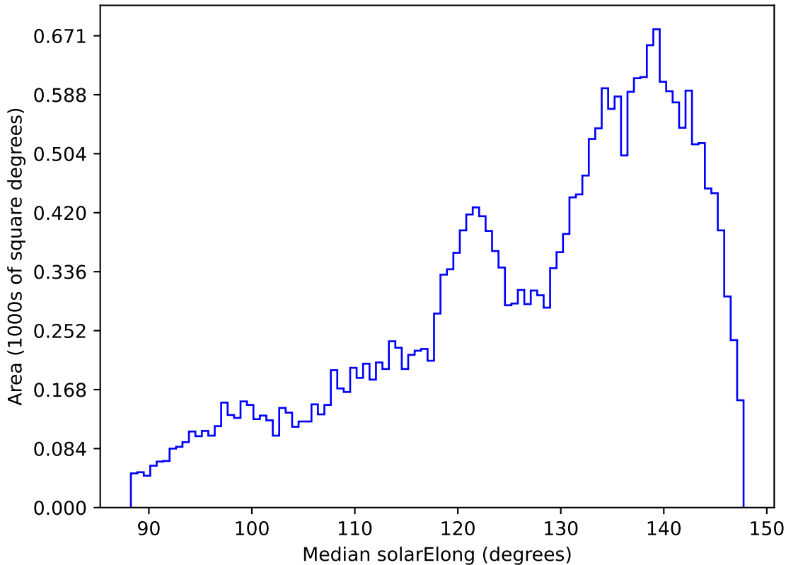
weather_cloudso12v3.4_10yrs All sky all bands: Median solarElong
