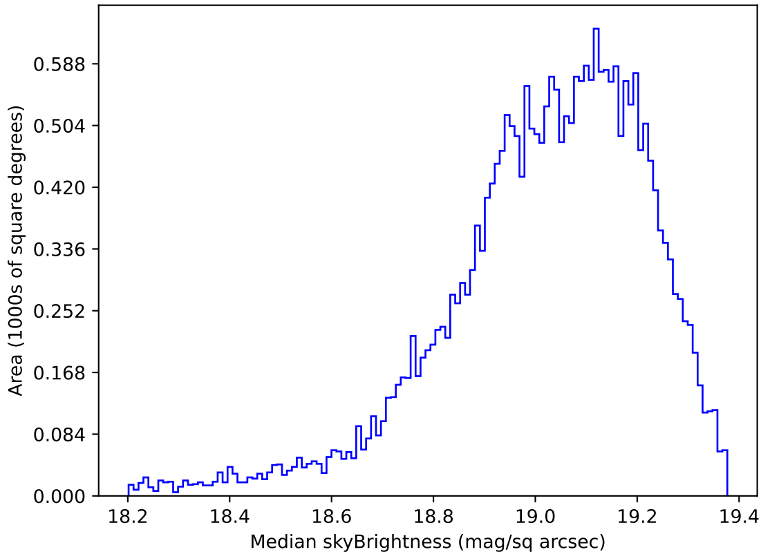
weather_cloudso12v3.4_10yrs Yr 1 z band: Median skyBrightness
