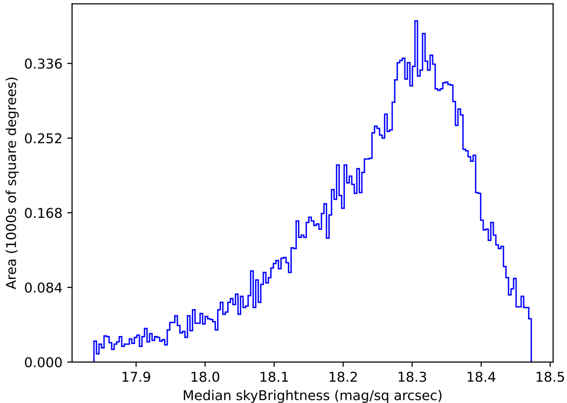
weather_cloudso12v3.4_10yrs Yr 1 y band: Median skyBrightness
