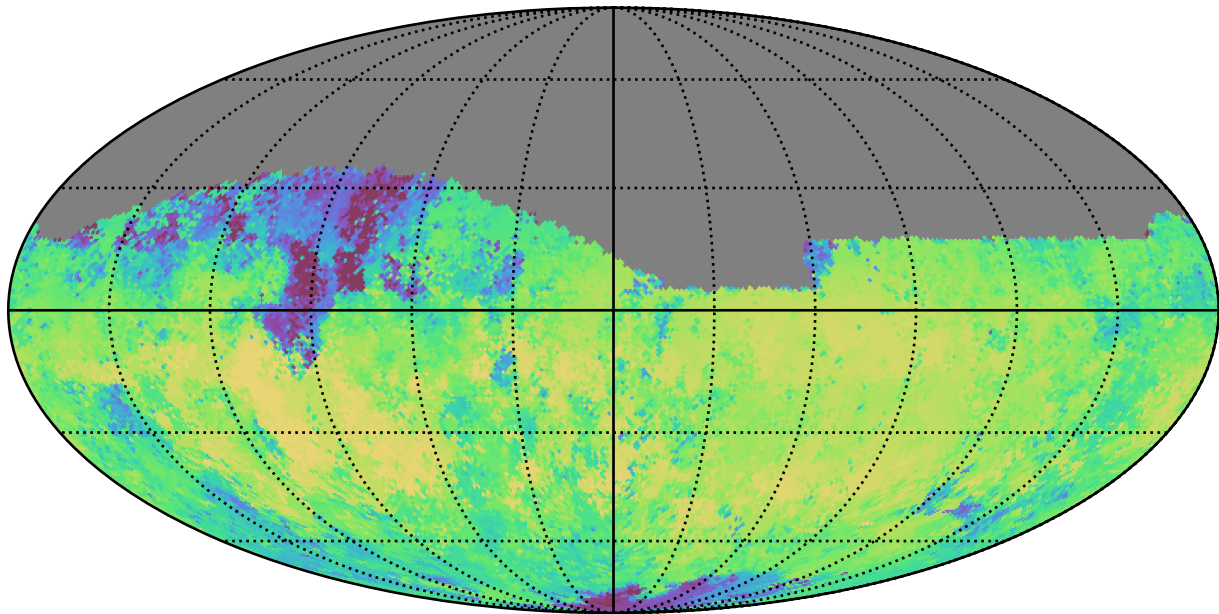
weather_cloudso12v3.4_10yrs Yr 1 i band: Median skyBrightness
