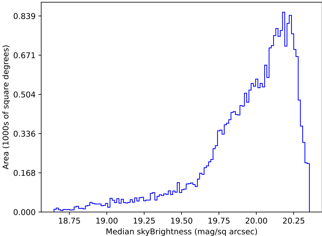
weather_cloudso12v3.4_10yrs Yr 1 i band: Median skyBrightness
