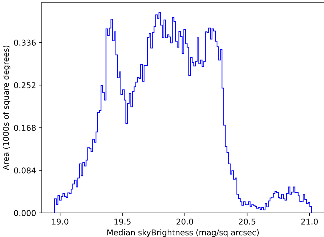
weather_cloudso12v3.4_10yrs Yr 1 all bands: Median skyBrightness
