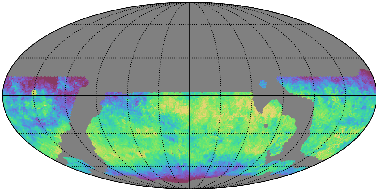
weather_cloudso12v3.4_10yrs WFD z band: Median skyBrightness
